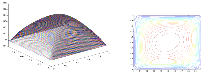
FIGURE 4. BFO iterative method on Test 3, h = 1/2^4 , d = 3 .
